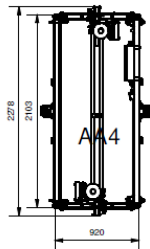
Configuration 11 Plate-forme 2100x920 0654210010
