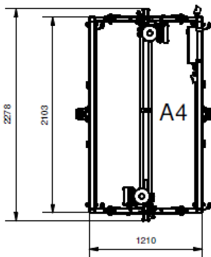
Configuration 10 Plate-forme 2100x1210 0654210009
